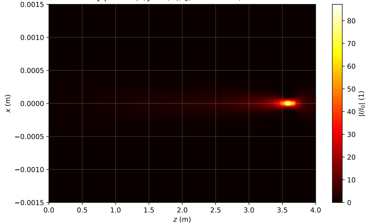
Intensity profile I(x, y = 0, z)/I_0 , P_{in}=1.1P_{cr} , artificial time
